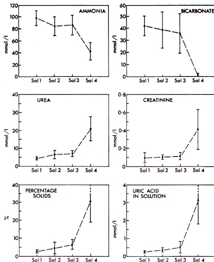
Fig. 3. Nitrogen excretion in liquid cloacal urine by C. porosus at different levels of salinity, and comparative percentages of solids in cloacal urine. Error bars are 95% confidence limits
