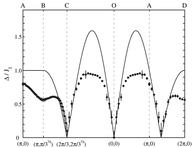
FIG. 1. Excitation spectrum for the TLM ( J_1 = J_2 ) along the path ABCOAQD shown in Fig. 4. The high-energy spectrum is strongly renormalized downwards compared to the LSWT prediction (solid line). Note the roton minima at B and D and the flat dispersion in the middle parts of CO and OQ.
