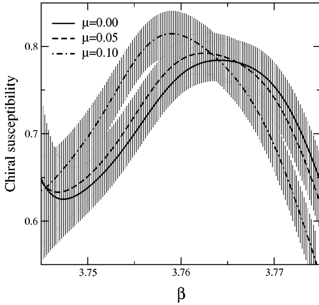
FIG. 12. \chi_{\bar{\psi}\psi}(\beta) at m=0.2 for various \mu .
