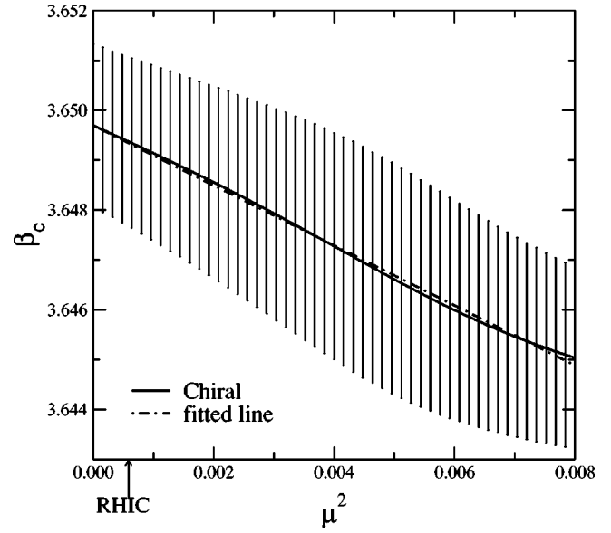
FIG. 14. Phase transition point \beta_c(\mu) determined by \chi_{\bar{\psi}\psi} at m=0.1 .
