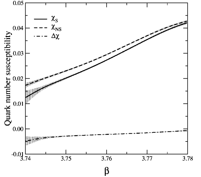
FIG. 23. Quark number susceptibilities \chi_S and \chi_{NS} at m=0.2 .
