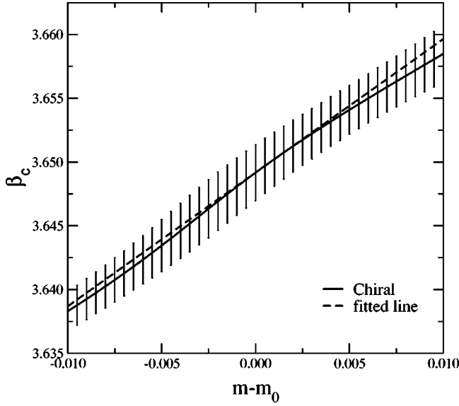
FIG. 6. \beta_c(m) determined by \chi_{\bar{\psi}\psi} around m=0.1 .
