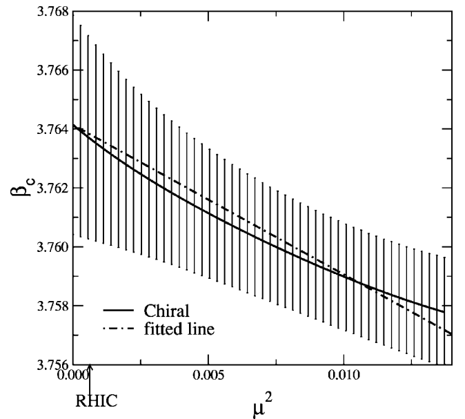
FIG. 15. Phase transition point \beta_c(\mu) determined by \chi_{\bar{\psi}\psi} at m=0.2 .
