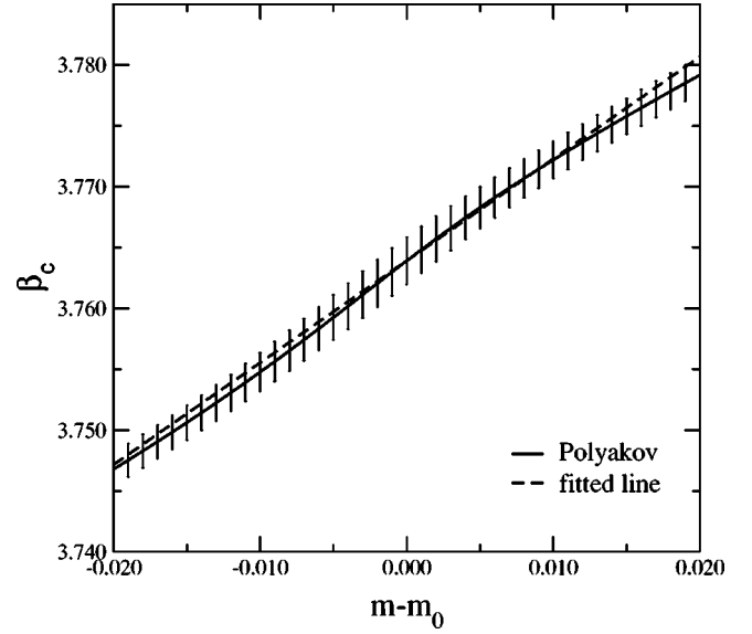
FIG. 5. \beta_c(m) determined by \chi_L around m=0.2 .
