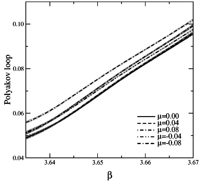
FIG. 17. L(\beta) at m=0.1 for various \mu .
