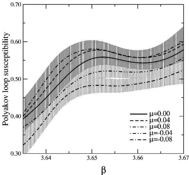
FIG. 9. \chi_L(\beta) at m=0.1 for various \mu .
