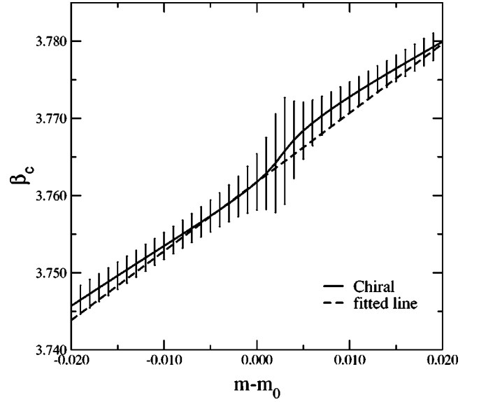
FIG. 7. \beta_c(m) determined by \chi_{\bar{\psi}\psi} around m=0.2 .
