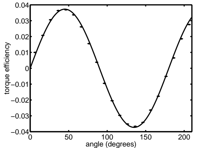
FIG. 3: Torque efficiency ( \hbar/\text{photon} ) vs angle between axis of glass rod of radius 0.67 \pm 0.03 \mu\text{m} and plane of polarization. Both experimental values obtained from polarization measurements and numerical calculations using our T -matrix model (solid line).
