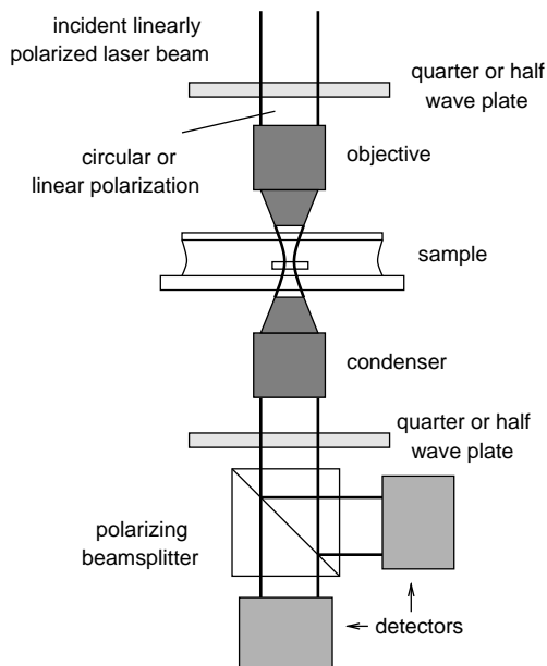
FIG. 1: Schematic diagram of optical tweezers setup showing where a half-wave plate can be added for alignment control, or a quarter-wave plate to produce a circularly polarized beam. The waveplate in front of the beamsplitter and detectors can be either a quarter-wave plate, to measure the polarization in a circular basis, or a half-wave plate, to measure it in a linear basis.
