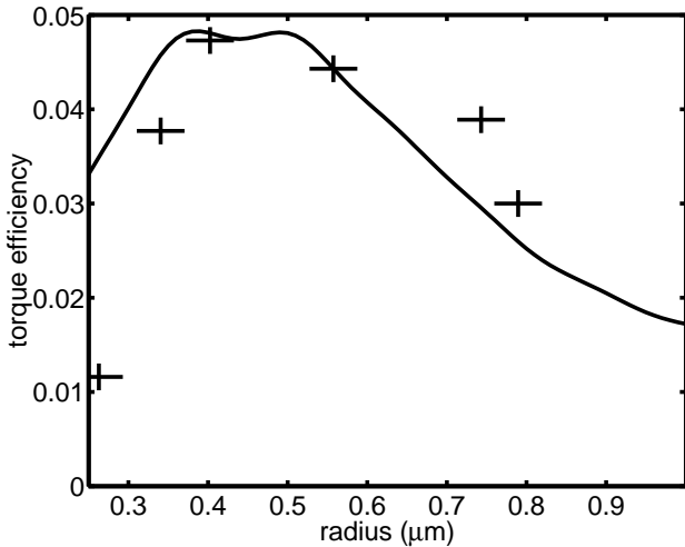
FIG. 4: Torque efficiency ( \hbar/\text{photon} ) vs radius for glass rods in a plane polarized beam. The angle between the rod axis and the plane of polarization is 45^\circ , giving the maximum torque. Both experimental values obtained from polarization measurements and numerical calculations using our T -matrix model (solid line) are shown.
