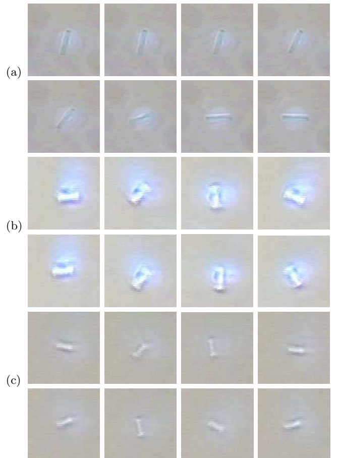
FIG. 2: Microscopic glass cylinders following rotating plane of polarization of trapping beam. The lengths of the cylinders are (a) 1.8 \mu\text{m} , (b) 2.6 \mu\text{m} , and (c) 5.5 \mu\text{m} . The frames are 0.04 s apart.
