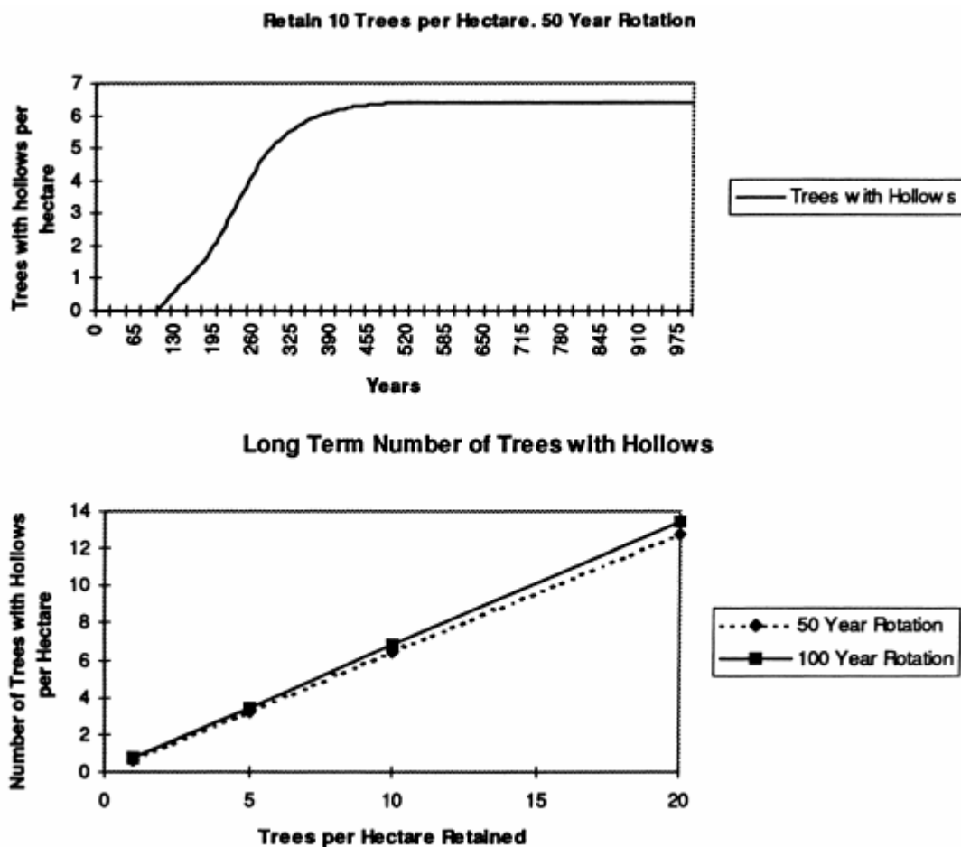
Fig. 8. Results from Scenario 2. (a) Time series from a single run. The logging regime has 10 trees ha -1 retained (with or without hollows) and a 50-year rotation. The first harvest occurs at 200 years. (b) The minimum number of trees with hollows per hectare in each rotation cycle after the simulation has stabilised. It is plotted against the number of trees retained.
