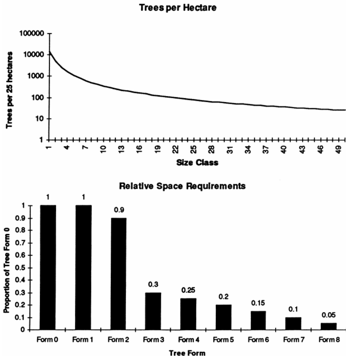
Fig. 5. Spatial requirements: (a) maximum number of Form 0 trees \text{ha}^{-1} (calculated from Ashton, 1976), and (b) the amount of space used or required by trees of different forms. These are given as a proportion of the amount of space a tree of Form 0 uses.
