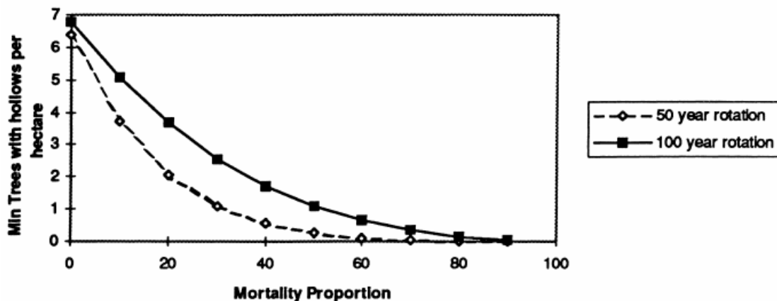
Fig. 9. Results from Scenario 3. The minimum number of trees with hollows per hectare which occur in a rotation cycle after a steady cycle has been reached. Mortality proportion is the proportion of trees which are to be retained, but collapse immediately following a tree-harvesting event.
