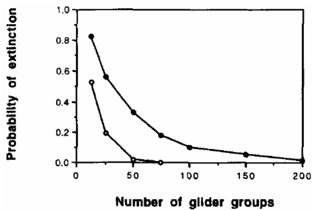
Fig. 5. Probability of extinction when the standard deviation in the environmental variation is varied.
